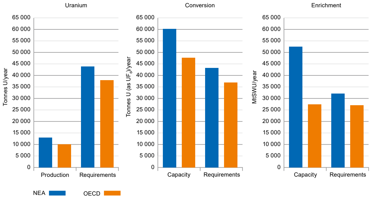
Figure 2.1: Fuel cycle supply and demand comparisons in OECD countries (as of 1 January 2021)
