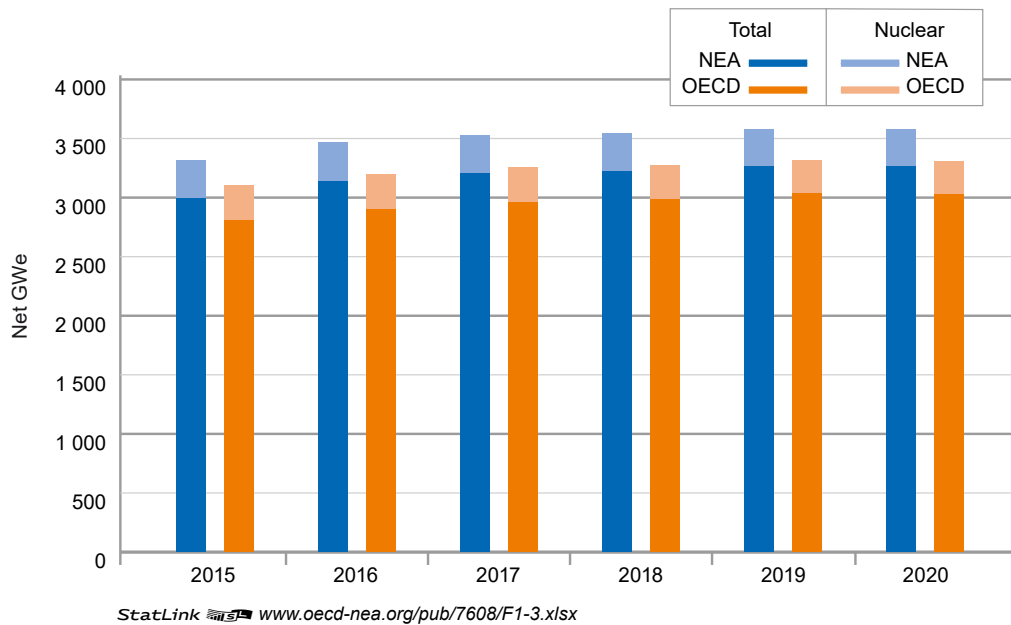
Figure 1.3: Trends in total and nuclear electricity capacity
