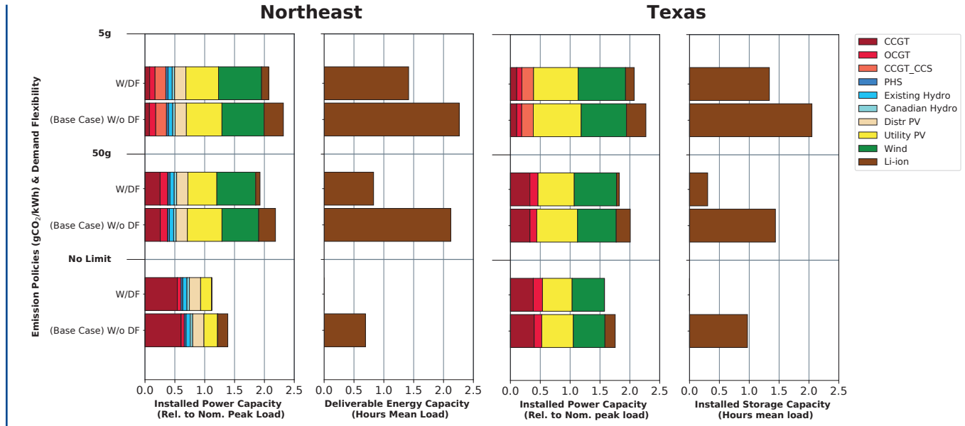
Figure 6.15 Impacts of demand flexibility in terms of installed power capacity, storage capacity, and SCOE, across a range of CO 2 constraints for the Northeast and Texas regions
