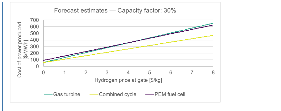
Figure 5.15 Forecast cost of power produced by technology vs. price of hydrogen at plant gate
