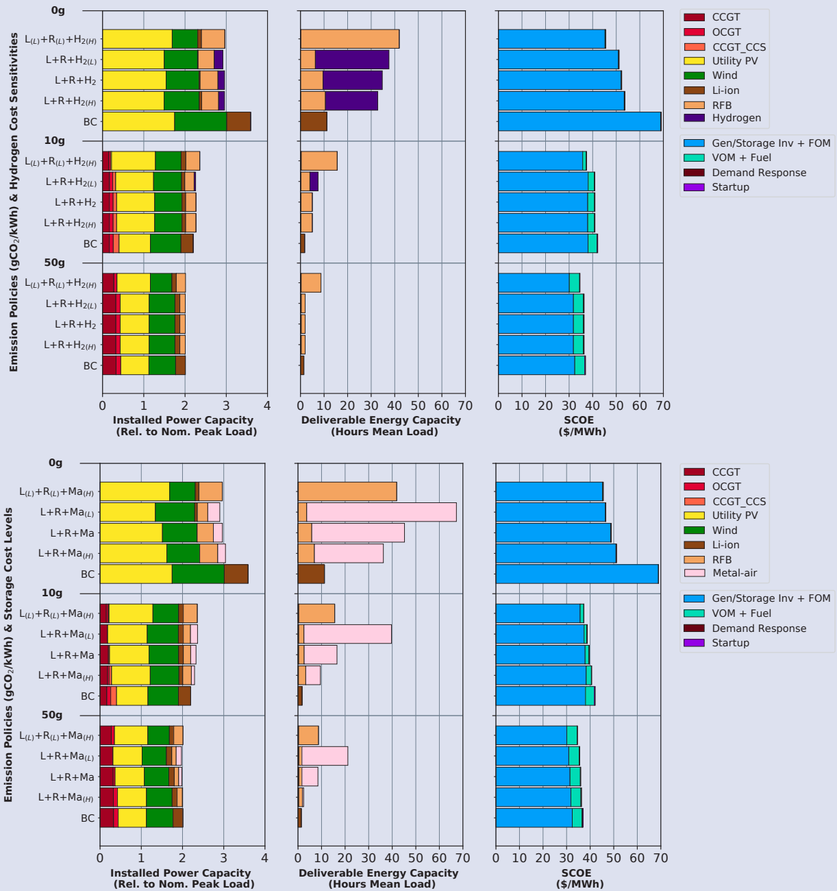
Figure C.8 System impacts of LDES availability at different assumed cost levels in Texas
