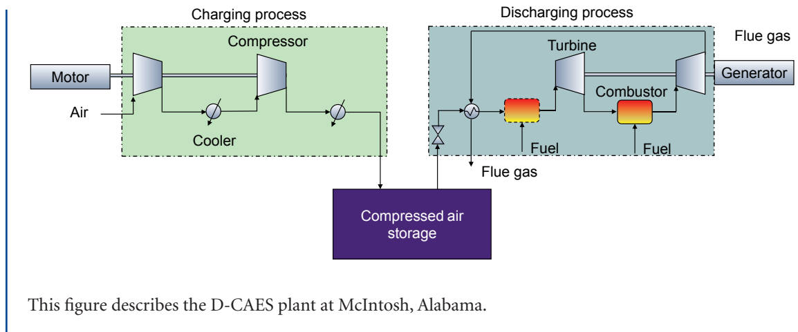
Figure 3.6 Flowsheet of a diabolic CAES system with a recuperator
