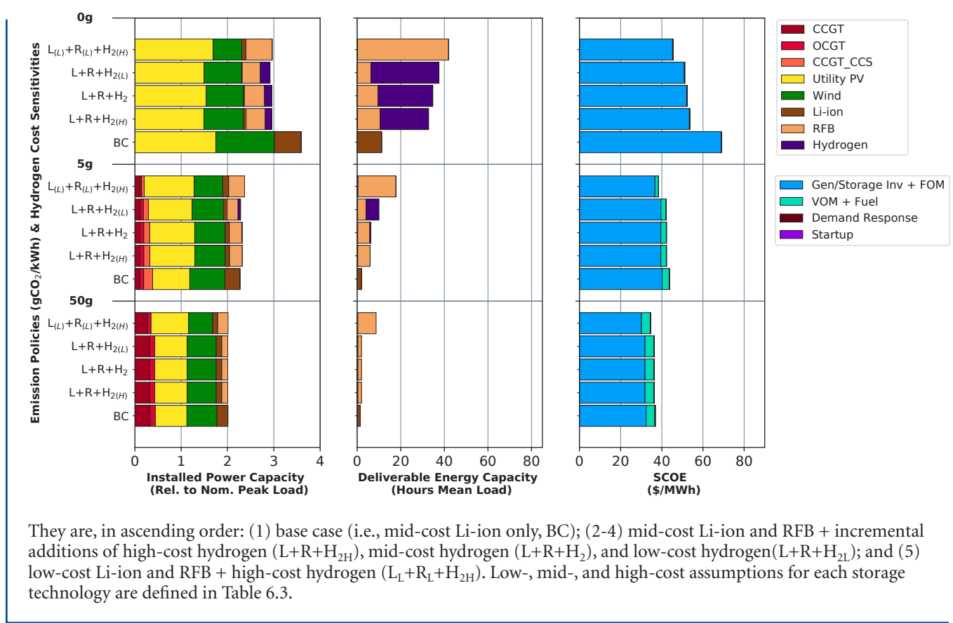
Figure 6.12 Impacts of low-, mid-, and high-cost hydrogen on installed power capacity, storage capacity, and SCOE, across a range of CO 2 constraints for the Texas region
