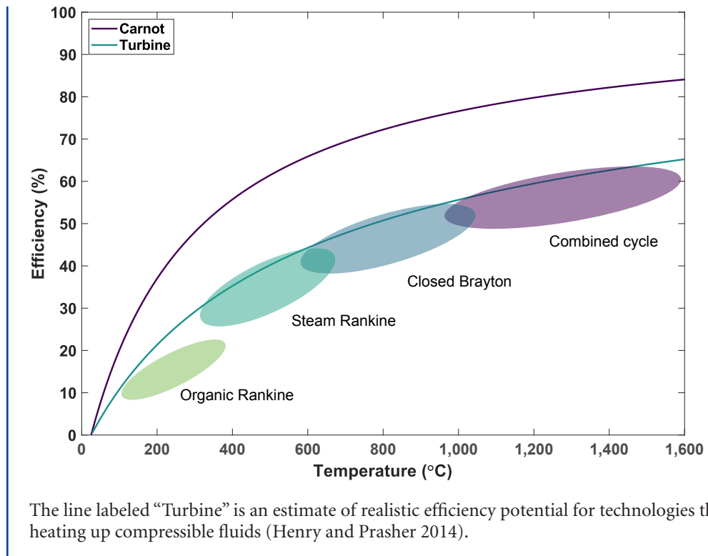
Figure 4.6 Approximate efficiencies of heat-to-electricity technologies plotted against Carnot efficiency
